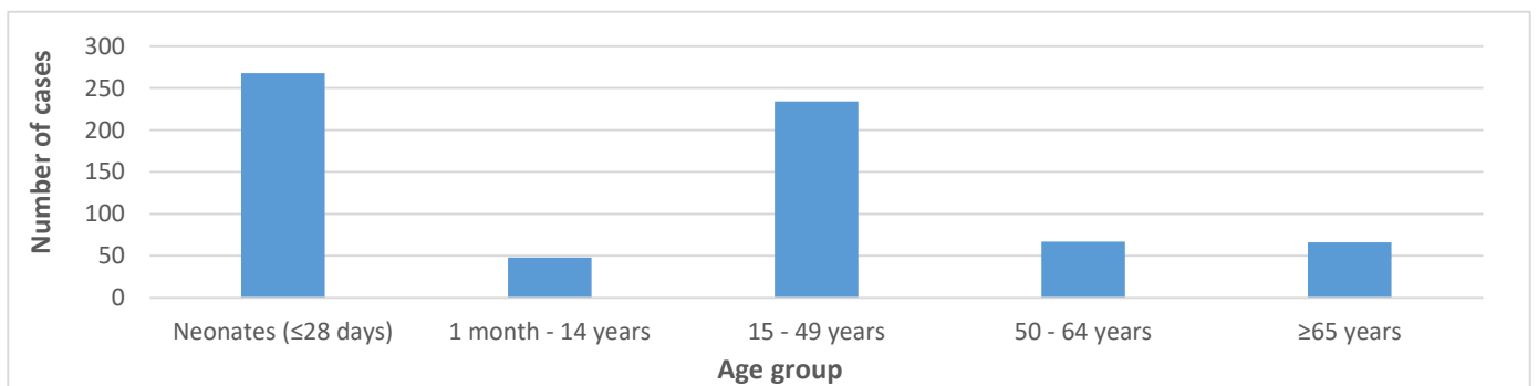
Figure 2: Age distribution of laboratory-confirmed listeriosis cases, South Africa, 01 January 2017 to 03 January 2018 (n=683)
